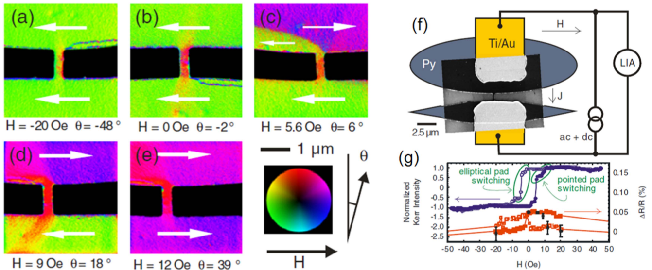
Figure 13. Measurement of spin-torque efficiency of a NiFe nanobridge by combining in situ STEM DPC Lorentz microscopy and magnetoresistance measurement [52]: (a)–(e) magnetisation configuration observed by DPC STEM LTEM at various applied field, (f) device structure for measurement and characterisation which was previously described in figures 9 and 10; (g) hysteresis loop and magnetoresistance results. Figure is reproduced under permission of AIP Publishing.
