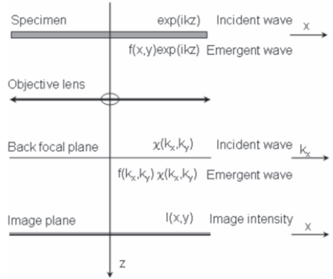
Figure 1. Image formation of magnetic structure in conventional TEM [12]. The figure is reproduced under permission of the thesis author (D-T Ngo).
