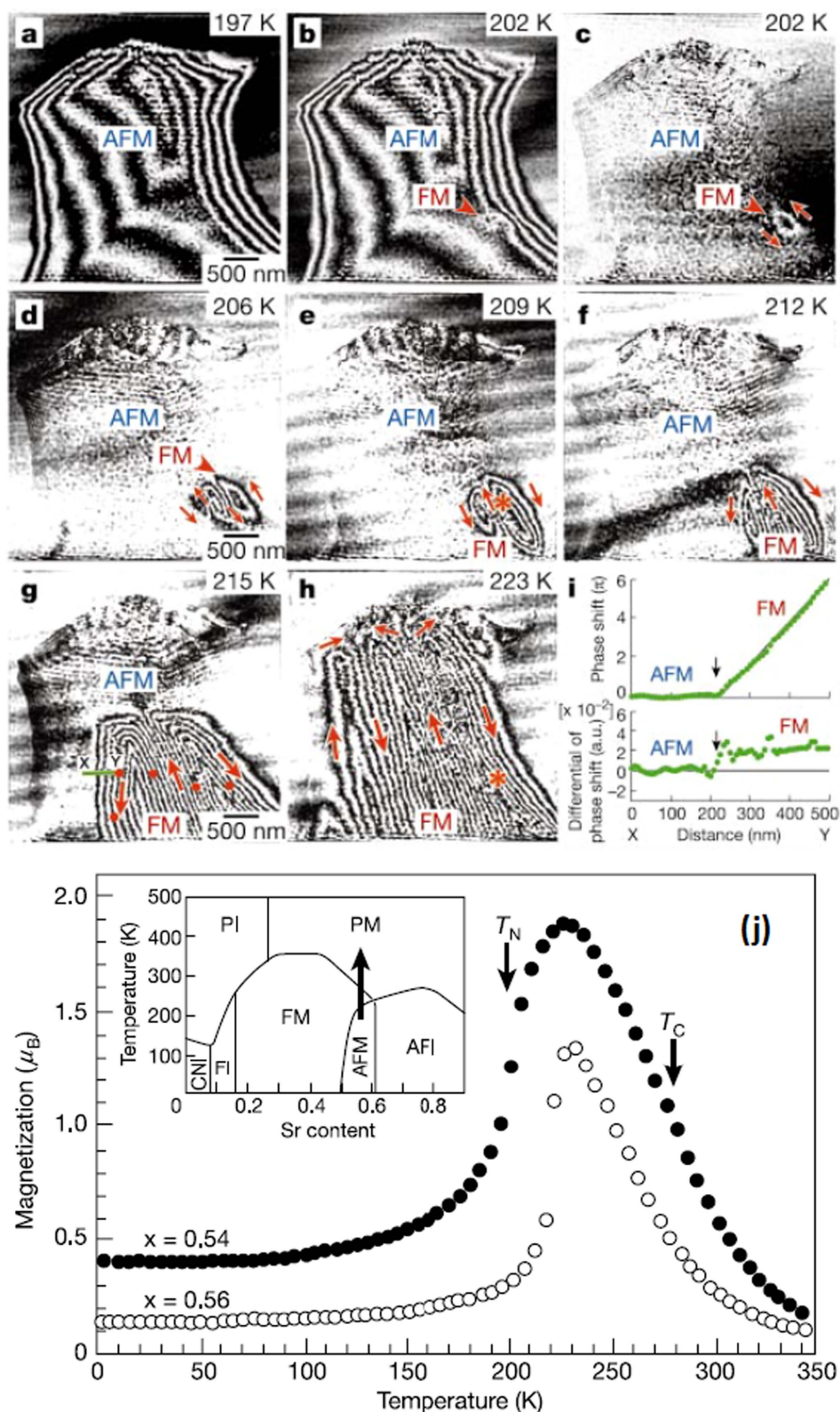
Figure 16. Temperature dependence of the magnetic microstructure in the mixed-phase (ferromagnetic and antiferromagnetic) state in \text{La}_{1-x}\text{Sr}_x\text{MnO}_3 [62]: (a)–(b) magnetic structure of the sample at various temperatures around Néel temperature. Direction of lines of magnetic flux (black-and-white lines in (c)–(h)) is indicated by red arrows. The upper panel of (i) illustrates the phase shift along the line X–Y in (g). The lower panel of (i) demonstrates the differential of the phase shift. The plots in (j) show temperature dependence of magnetisation. The figure is reproduced under permission of Nature Publishing.
