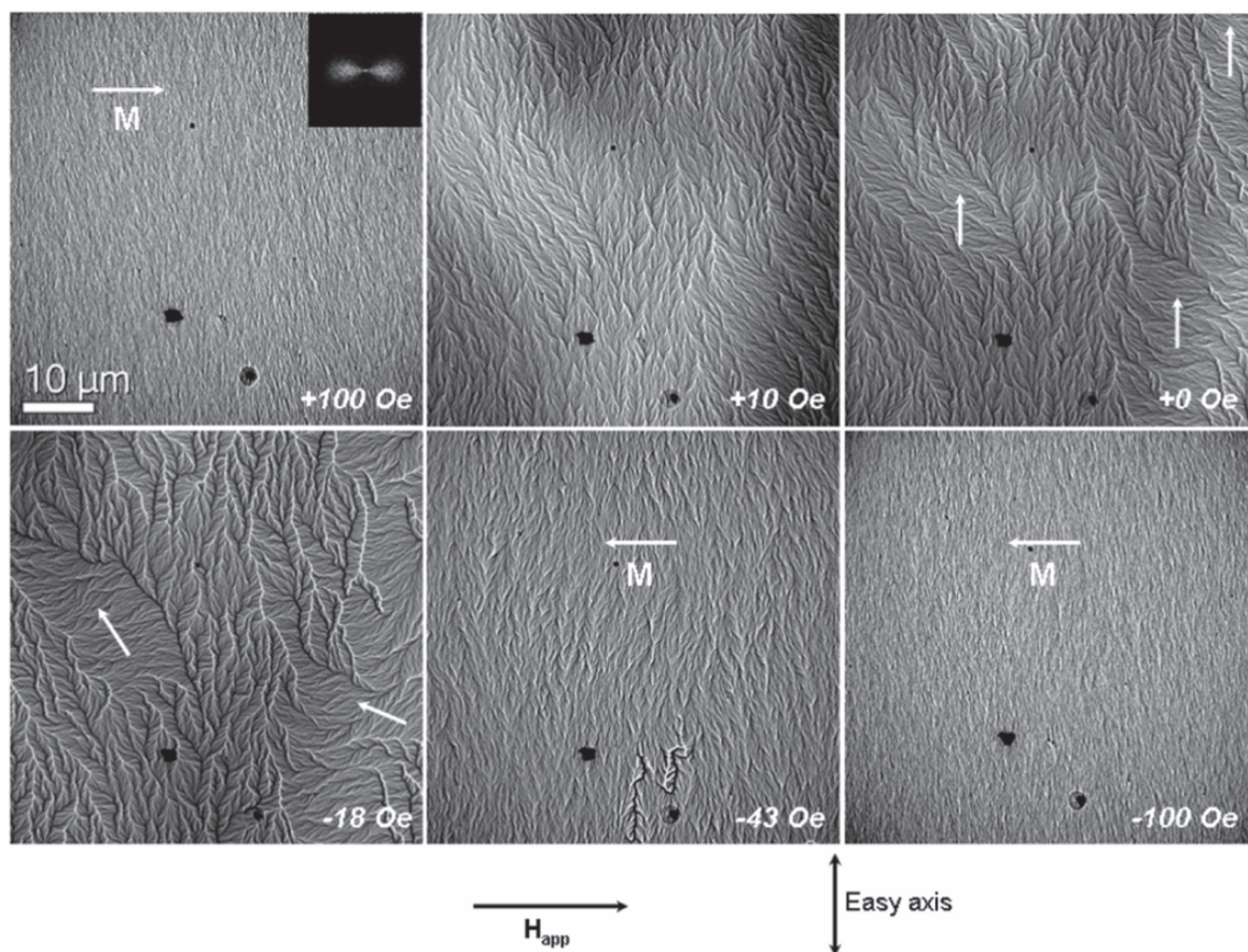
Figure 7. In situ LTEM study of magnetisation reversal in \text{Co}_{80}\text{Ir}_{20} film: Fresnel images in a hysteresis sequence on the hard axis in plane of the film. The images were recorded in a Philip CM20 TEM with a FEG [37]. The figure is reproduced under permission of IOP Publishing.
